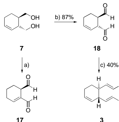
Scheme 6. Synthesis of bis-iodovinyl fragment 3 . a) (\text{COCl})_2 , \text{DMSO} , \text{CH}_2\text{Cl}_2 , -78^\circ\text{C} , 2 h; then \text{NEt}_3 , -78 \rightarrow -10^\circ\text{C} ; b) (\text{COCl})_2 , \text{DMSO} , \text{CH}_2\text{Cl}_2 , -78^\circ\text{C} , 1.5 h; then i\text{Pr}_2\text{NEt} , -78 \rightarrow -10^\circ\text{C} ; c) \text{CrCl}_2 , \text{CHI}_3 , \text{THF} , 0^\circ\text{C} \rightarrow \text{RT} , 2 h.
